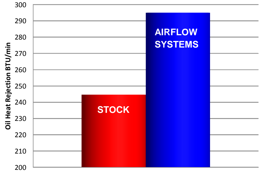
Oil Heat Rejection (20.5% Increase)
